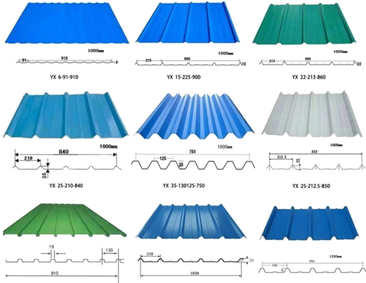
Trapezoidal roofing sheet
